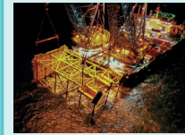
EPCI awarded for Seagreen's onshore and offshore HVAC substations
